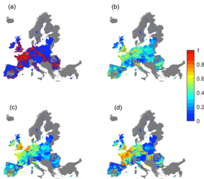
Figure 3.11: (a) Recorded groundwater chemical status (blue good, red poor); modelled status (b) based on agricultural area, population and precipitation; (c) based on agricultural area, population and precipitation with countries as a fixed effect; and, (d) based on stepwise regression of all variables.
