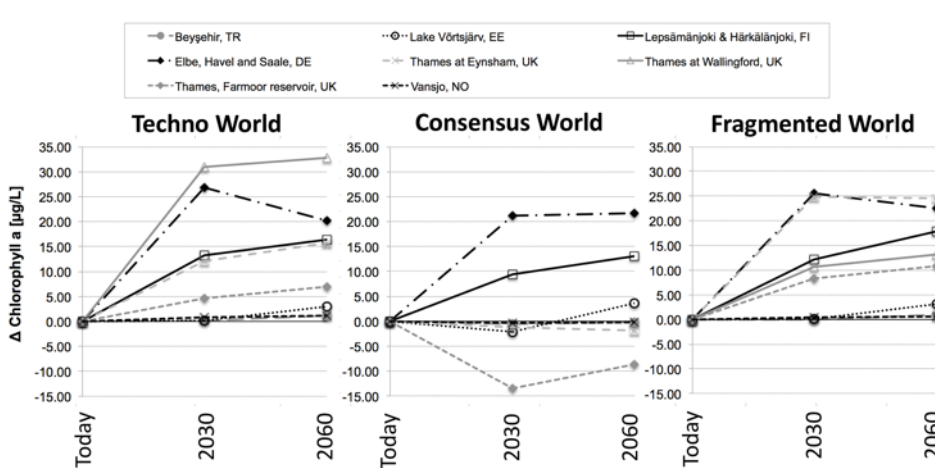
Figure 3.8: Relative change in Chlorophyll-a concentrations for the future scenarios across eight case-studies.
