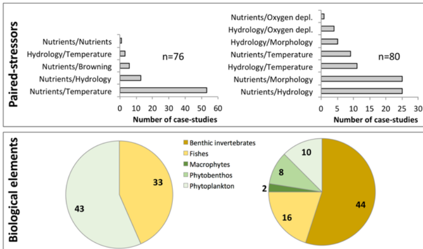
Figure 3.17: Summary of case studies contributing to the synthesis analysis indicating the stressor combinations studied and the biological responses, broken down by lakes [left] and rivers [right].
