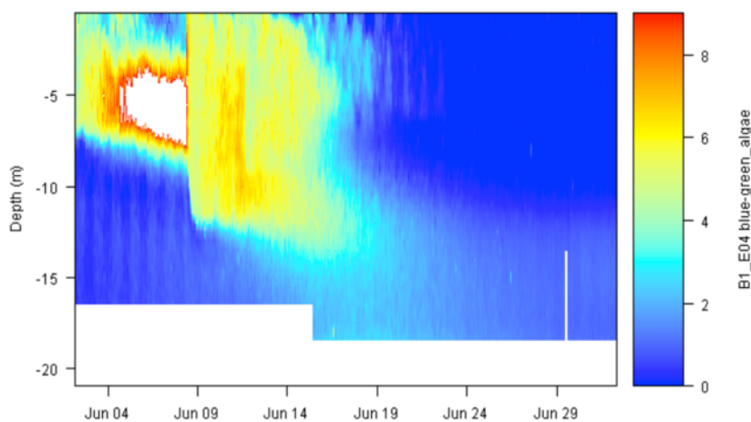
Figure 3.4: Cyanobacteria biomass estimated from fluorescence measurements in the mesocosm with medium addition of humic substances. This mesocosm received no extra nutrients.
