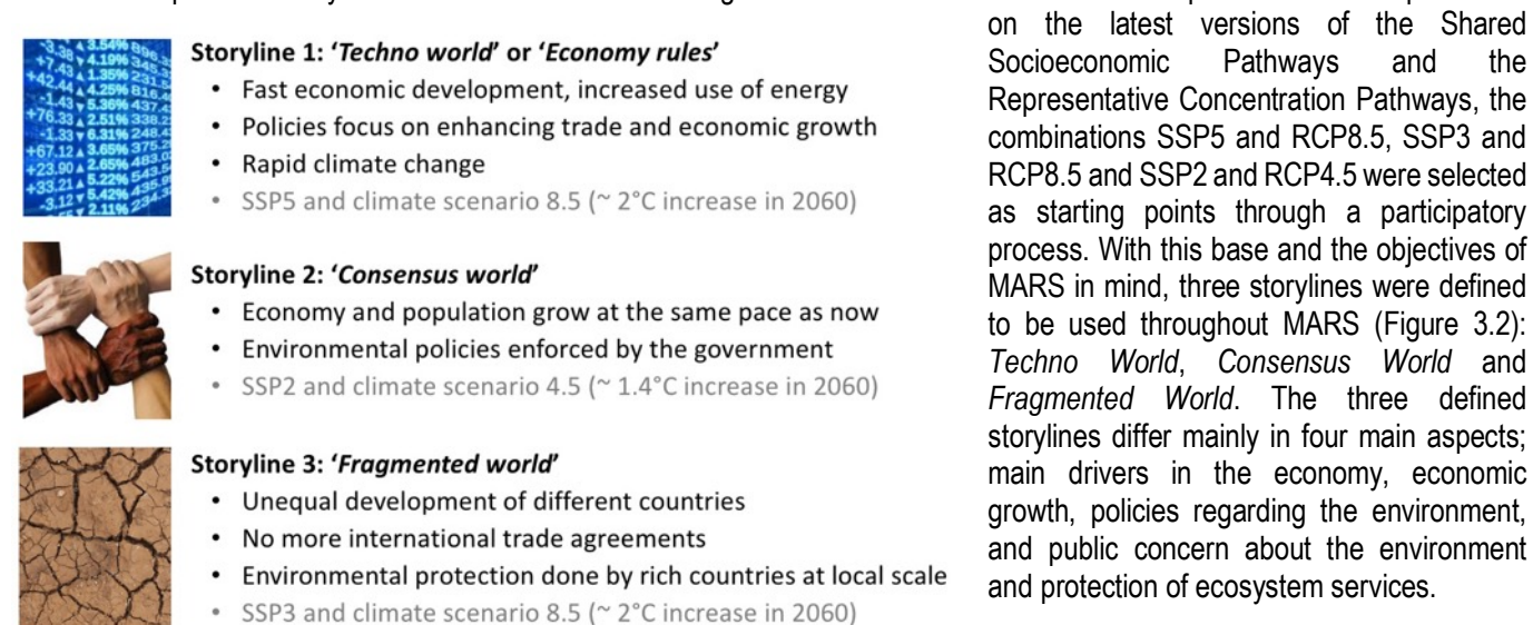
Figure 3.2: Features of the three storylines developed in MARS.
